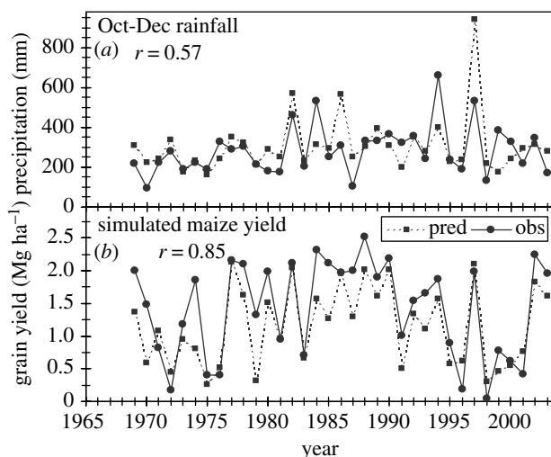
Figure 2. (a) Predicted and observed October–December rainfall and (b) simulated maize yields, Katumani, Kenya. Maize yields are from APSIM run with 20 realizations of stochastic rainfall disaggregated from monthly hindcasts, 40 kg ha -1 applied N fertilizer, stand density of 3.5 m -2 (courtesy of K. P. C. Rao, ICRISAT Nairobi). Maize yields simulated with observed rainfall serve as the benchmark for comparison. Rainfall hindcasts are based on a linear transformation of ECHAM four simulations, forced with observed SST boundary conditions ( Hansen & Indeje 2004 ).
