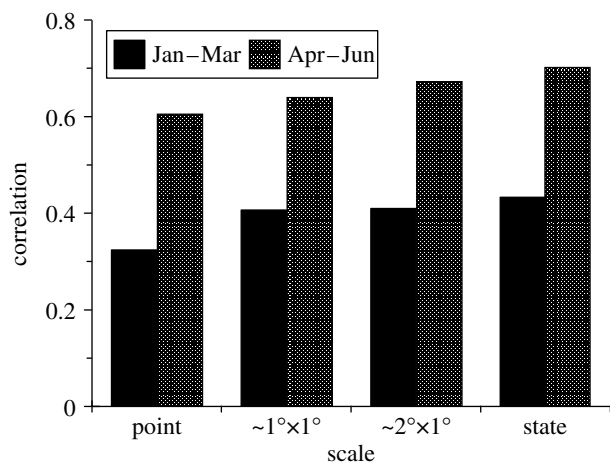
Figure 1. Correlation of observed versus predicted rainfall in the state of Ceará, northeast Brazil, as a function of scale of aggregation. Source: Gong et al. 2003 .
